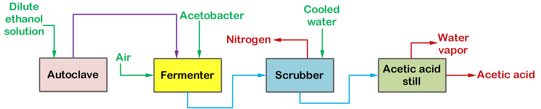
Figure: Manufacture of acetic acid by oxidative fermentation
